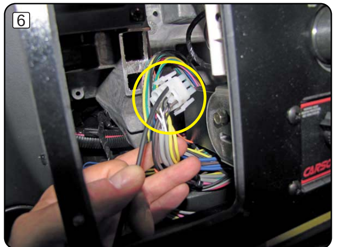
Connect the new black wire in position 9 of the switchplex connector. (see drawing # 1)
