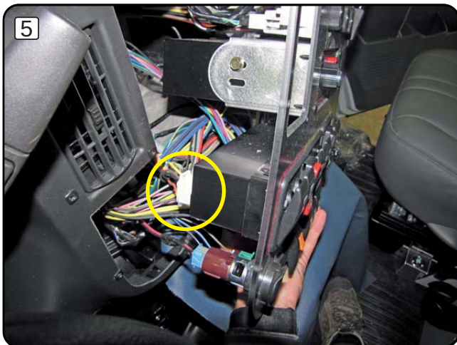
Locate the 9 position connector connected behind the switchplex as shown.
