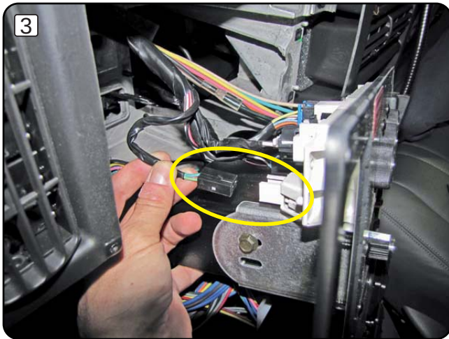
Locate the 2 position connector with the green wire and the light green wire connected behind the gm climate control module as shown.
