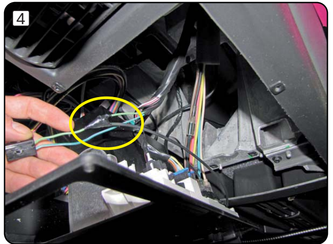
Weld the new black wire with the light green wire . Insulate the soldering with electrical tape. (see drawing # 1)
